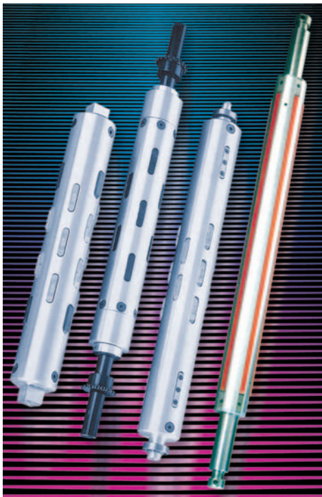
Single and multi bladder airshafts with continuous and intermittent lug designs.
